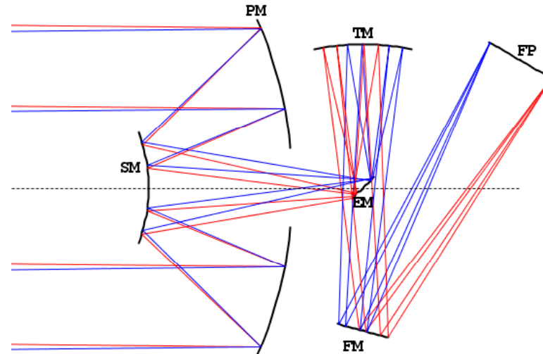
Korsch full-field configuration II
