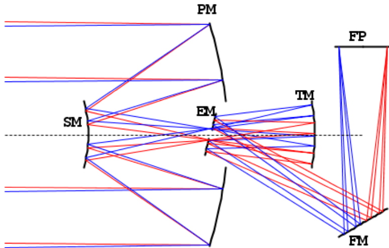
Korsch full-field configuration I
