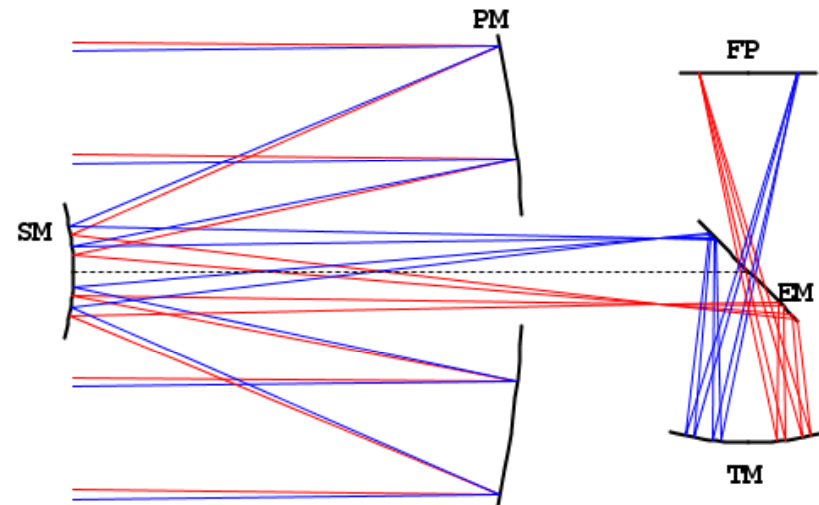
Korsch annular-field configuration II
