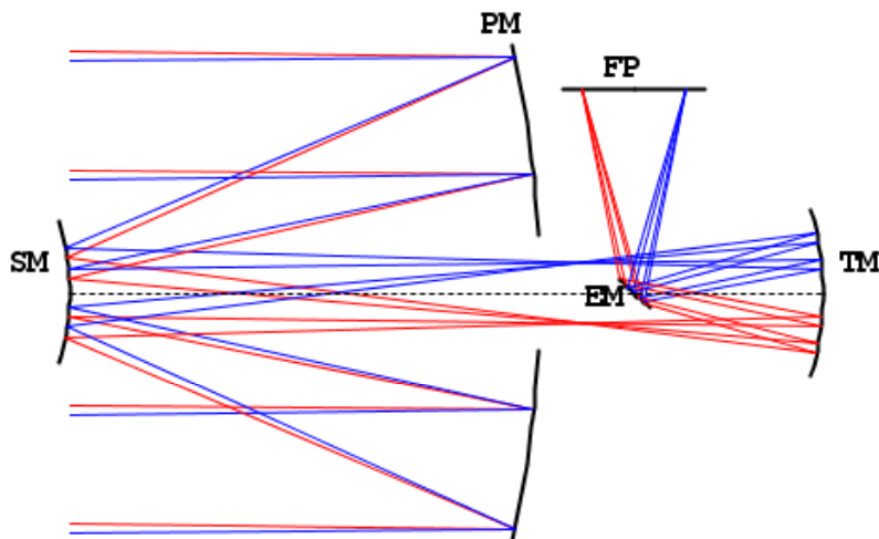
Korsch annular-field configuration I
