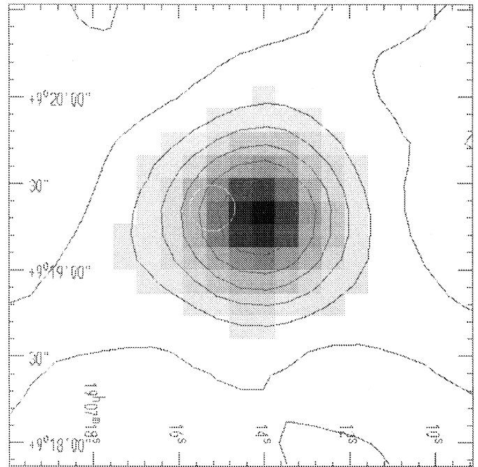
FIG. 3.—Enlargement of the area around source 1. The two infrared sources in Vrba et al. (1996) are located at the center of the circle.
