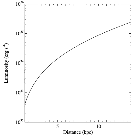
FIG. 2.—Source luminosity as a function of assumed distance. The total column density in this direction, 10^{22} \text{ cm}^{-2} (determined using the HEASARC on-line service) along a line of sight of 14 kpc, has been scaled linearly to the distance.
